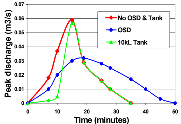
Figure 7. Hydrographs of stormwater discharge from rainwater tanks and OSD from a single storm event
